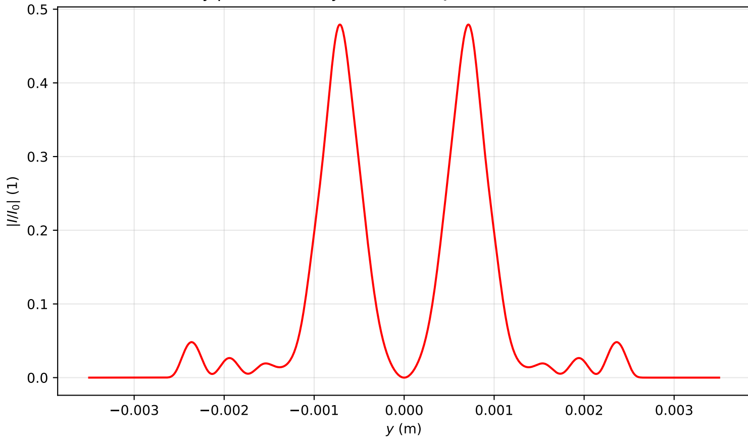
Intensity profile I(x = 0, y, z = 2.946)/I_0 , P_{in}=6.0P_{cr} , artificial time
